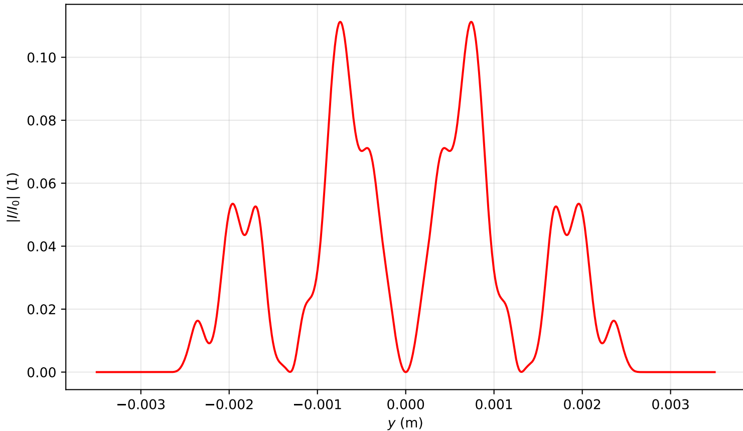
Intensity profile I(x=0, y, z=2.707)/I_0 , P_{in}=9.0P_{cr} , artificial time
